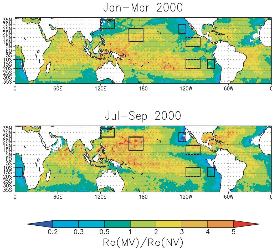
Figure 4. Ratio of R_{e(MV)} to R_{e(NV)} in three-monthly mean in JFM (upper) and in JAS (lower) 2000. Boxes shown in the figure indicate the sites listed in Table 1.
