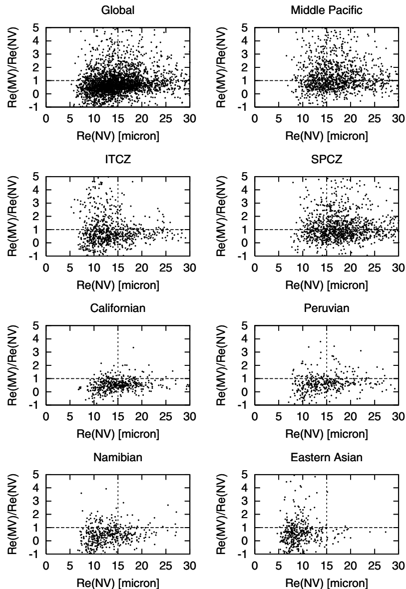
Figure 6. Ratio of R_{e(MV)} to R_{e(NV)} versus R_{e(NV)} in JFM 2000. Location of each site is listed in Table 1.
