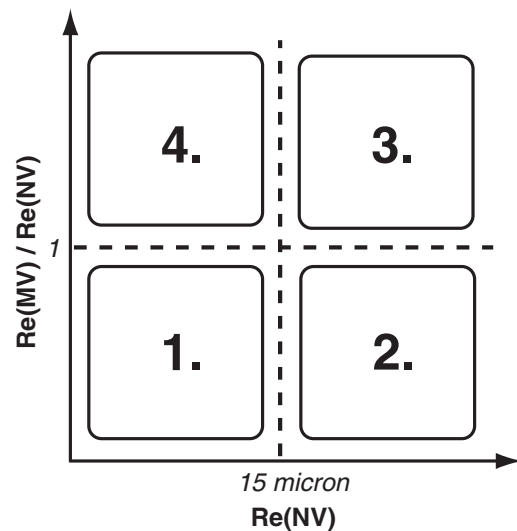
Figure 5. A schematic illustration to categorize the microphysical status of low clouds (see section 3.3 for details).
