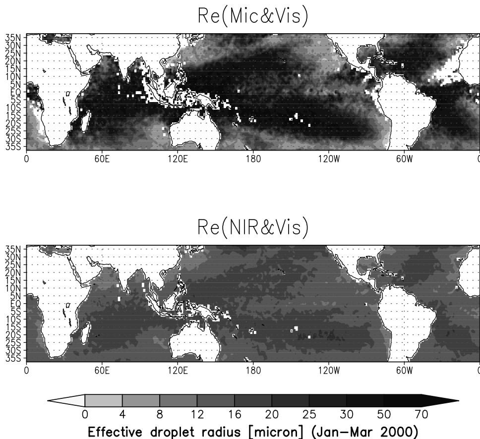
Figure 8. Three-monthly mean (top) R_{e(MV)} and (bottom) R_{e(NV)} for January to March 2000. See color version of this figure at back of this issue.
