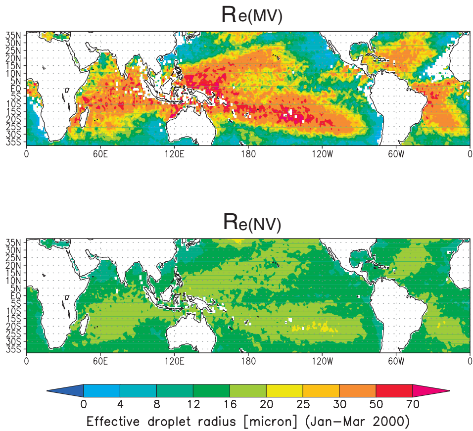
Figure 8. Three-monthly mean (top) R_{e(MV)} and (bottom) R_{e(NV)} for January to March 2000.
