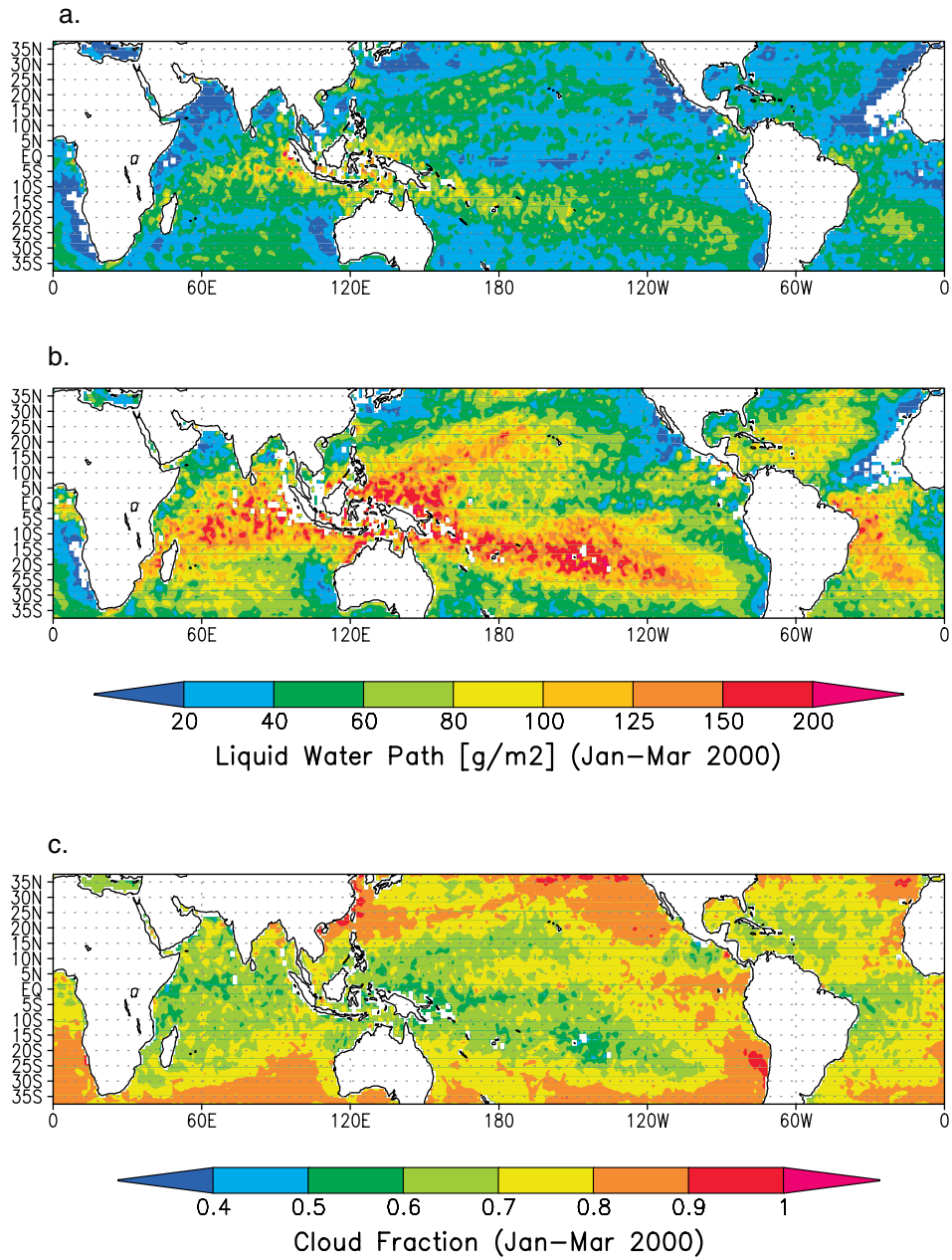
Figure 5. Three-monthly mean LWP_{mic} (a) without the cloud fraction correction, (b) with the correction, and (c) the cloud fraction for January to March 2000.
