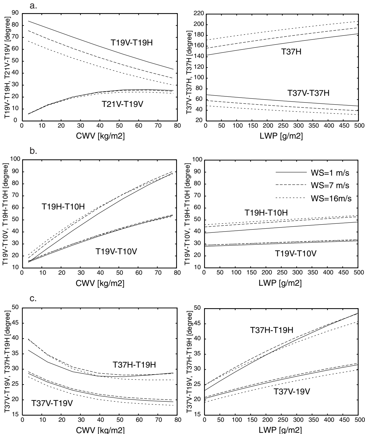
Figure 1. Calculated brightness temperatures as functions of columnar water vapor (CWV) or liquid water path (LWP). (a) T_{21V} - T_{19V} and T_{19V} - T_{19H} as functions of (left) CWV and T_{37V} - T_{37H} and T_{37H} as functions of (right) LWP. (b) T_{19V} - T_{10V} and T_{19H} - T_{10H} as functions of (left) CWV and of (right) LWP. (c) T_{37V} - T_{19V} and T_{37H} - T_{19H} as functions of (left) CWV and (right) of LWP. Solid, dashed, and dotted lines correspond to wind speeds (WS) of 1, 7, and 16 m/s, respectively.
