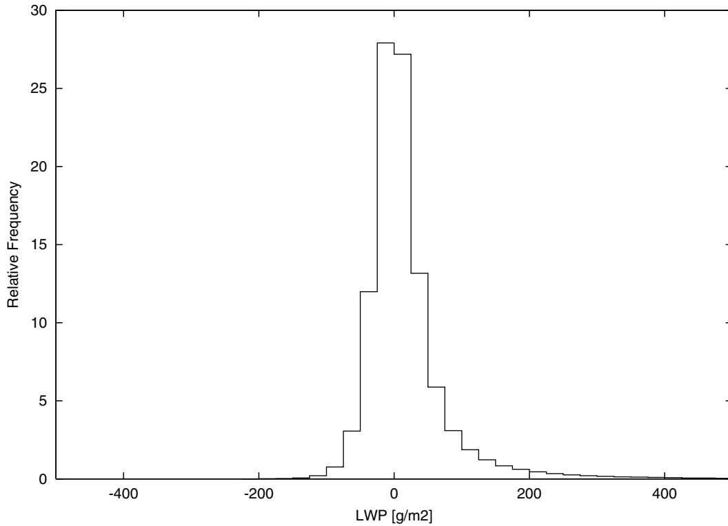
Figure 4. Frequency distribution of microwave-retrieved LWP ( LWP_{\text{micr}} ) for clouds with the optical thickness < 3 . The ordinate is the relative frequency in the unit of percent, and the abscissa is LWP_{\text{micr}} .
