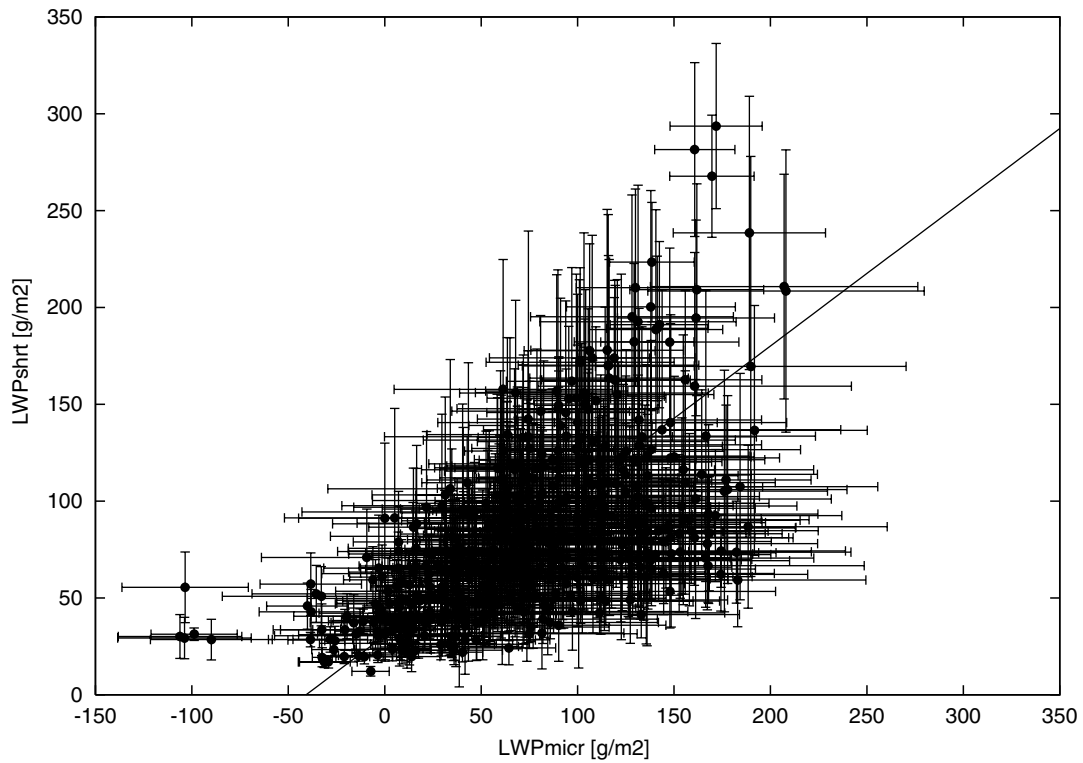
Figure 6. Scatterplots between LWP_{micr} (abscissa) and shortwave-retrieved LWP ( LWP_{shrt} ; ordinate) over the globe. Each plot and the associated error bars correspond to the average and the standard deviations, respectively, within a grid box of 2.5^\circ \times 2.5^\circ . The solid line delineates the linear fitting curve, given by LWP_{shrt} = 31 + 0.75LWP_{micr} g/m^2 . The correlation coefficient is 0.61.
