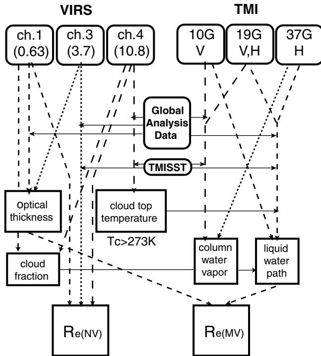
Figure 2. Overall flow of the combined algorithm is illustrated. VIRS and TMI denote the Visible and Infrared Scanner and TRMM Microwave imager, respectively. R_{e(NV)} is the cloud effective radius retrieved from near-infrared and visible radiances, and R_{e(MV)} is that which is retrieved from the microwave and the visible. TMISST as the TMI-retrieved sea surface temperature, which is provided by the Earth Observation Research Center (EORC) of the National Space Development Agency of Japan (NASDA). See section 2.3 for more detail.
