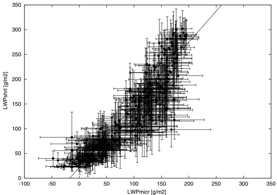
Figure 7. Same as Figure 6, but with the target area a rectangular region of 15^\circ S - 30^\circ S and 75^\circ W - 85^\circ W in western Chile. The linear fitting curve is given by LWP_{shrt} = 22 + 1.26 LWP_{micr} (g/m^2) with a correlation coefficient of 0.91.
