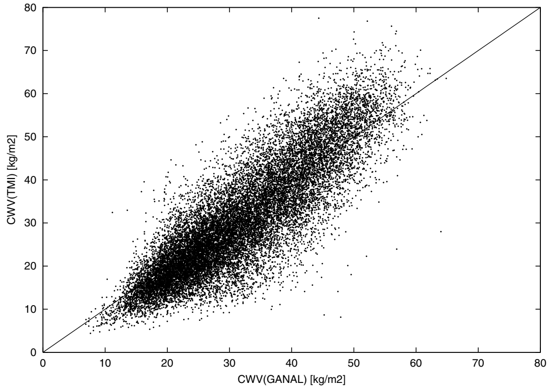
Figure 3. Scatterplot for the TRMM Microwave Imager (TMI)-retrieved CWV (ordinate) versus CWV calculated from global analysis (GANAL) (abscissa).
