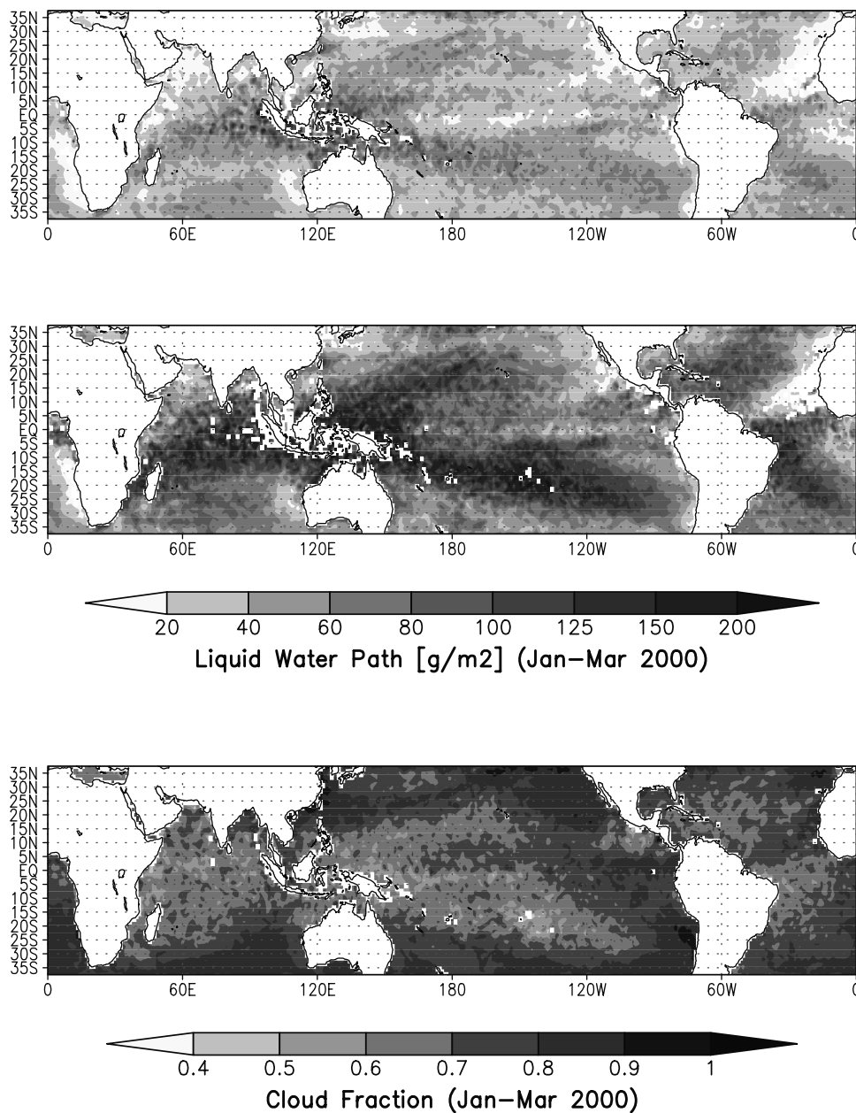
Figure 5. Three-monthly mean LWP_{micr} (a) without the cloud fraction correction, (b) with the correction, and (c) the cloud fraction for January to March 2000. See color version of this figure at back of this issue.
